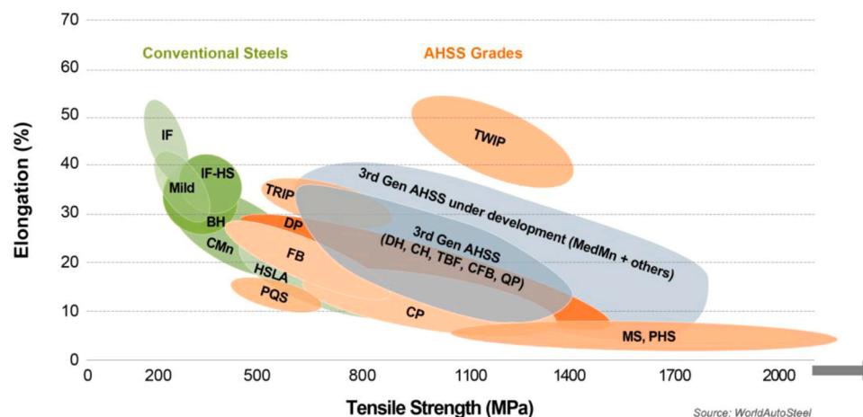
Fig. 25. Relation between strength and elongation of current and emerging steel grades (image source: www.worldautosteel.org ).
