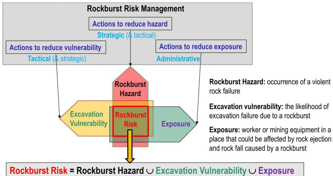
Fig. 5. Rockburst risk and its three routes. Rockburst risk is the union (indicated by \cup in the equation) of rockburst hazard, excavation vulnerability, and exposure.
