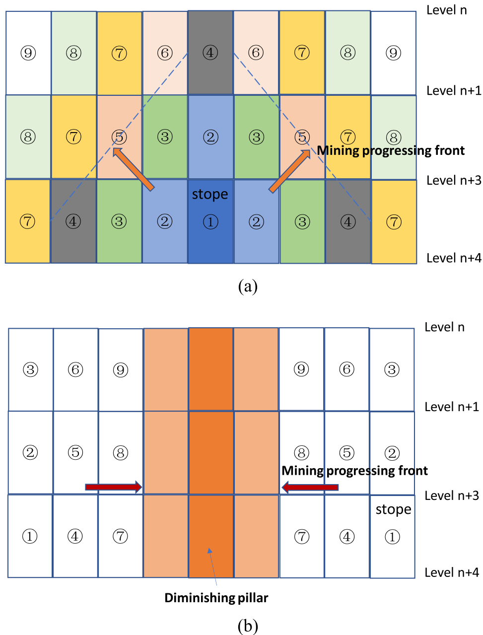
Fig. 12. (a) Bottom-up "chevron" mining sequence; (b) mining sequence leading to diminishing pillar.
